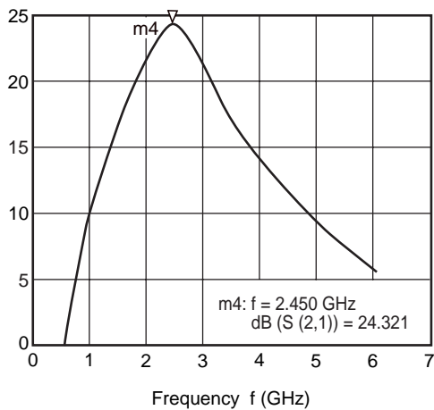
S21-FREQUENCY
