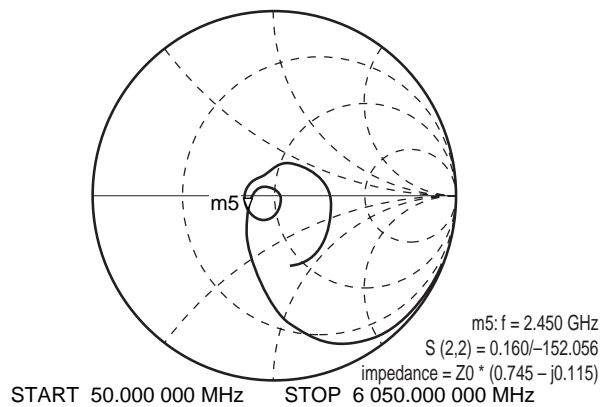
S22-FREQUENCY
